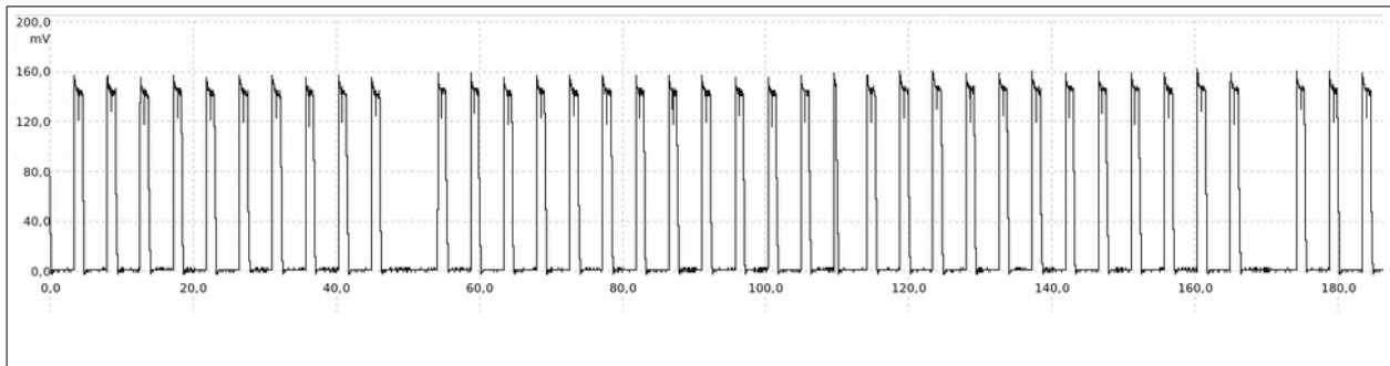
Figur 13: Signalstrukturplot for en GSM-forbindelse. Pulsinterval 4,62ms, pulsvarighed: 0,57ms.
